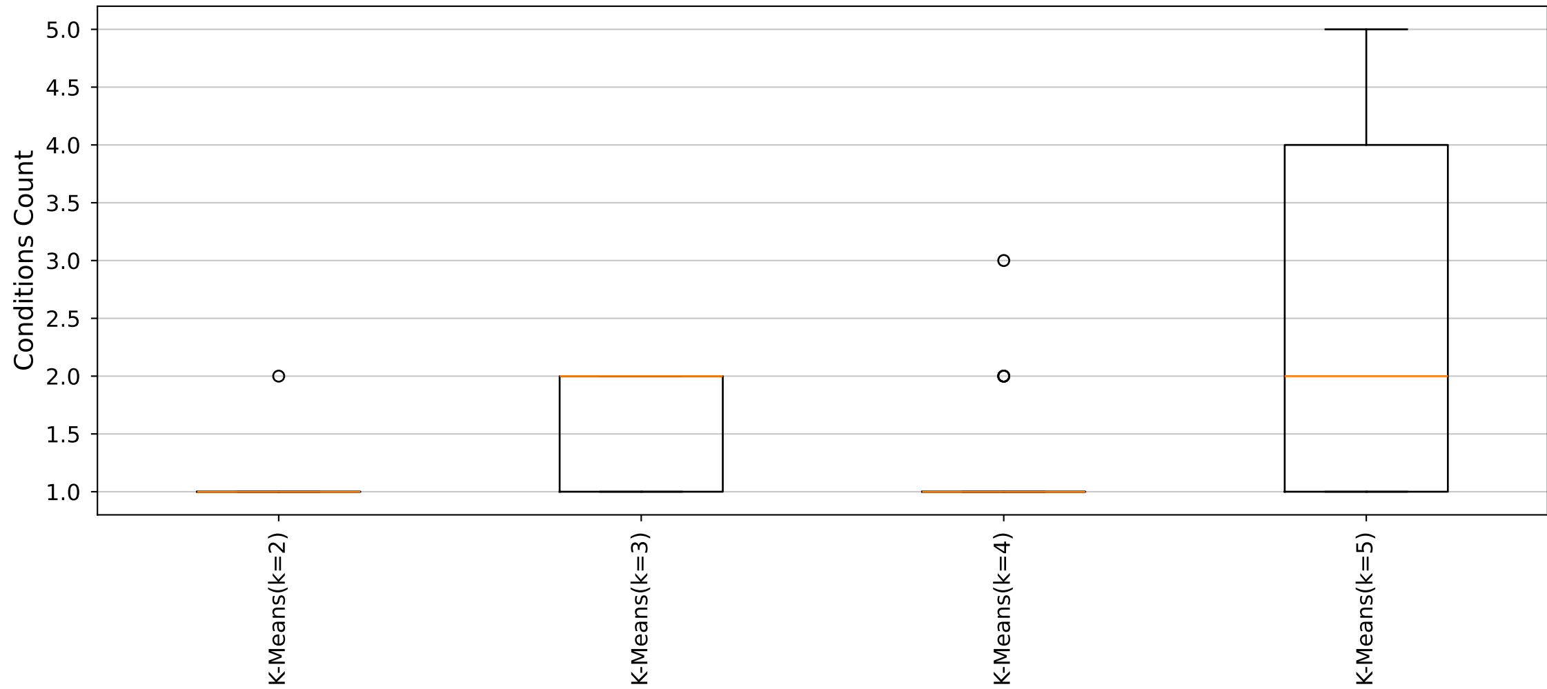
YARA Rules Conditions Count Distribution (Cluster36_Size5 dataset)
